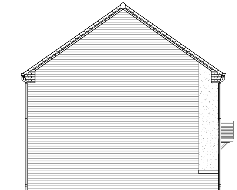
Left Elevation
